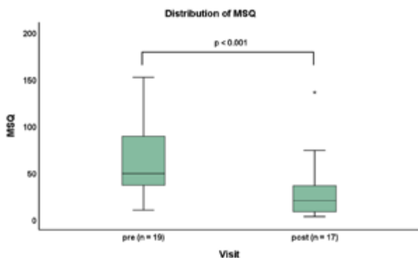
Figure 1 Distribution of MSQ p-value of Wilcoxon test for paired samples (n = 17)
